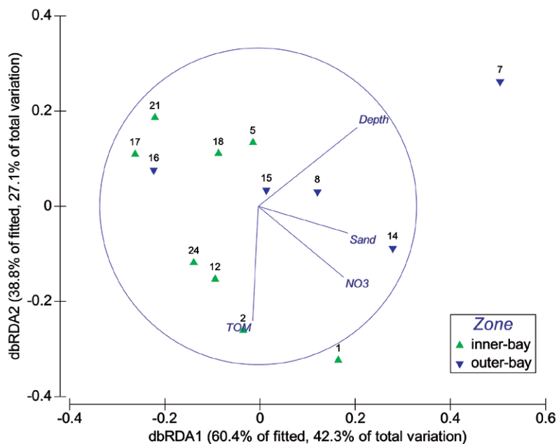
Figure 6. RDA projection biplot based on Spearman-rank measure of fourth root taxa abundances. Numbers indicate sampling sites. Only environmental predictors selected by the forward selection model are shown.
